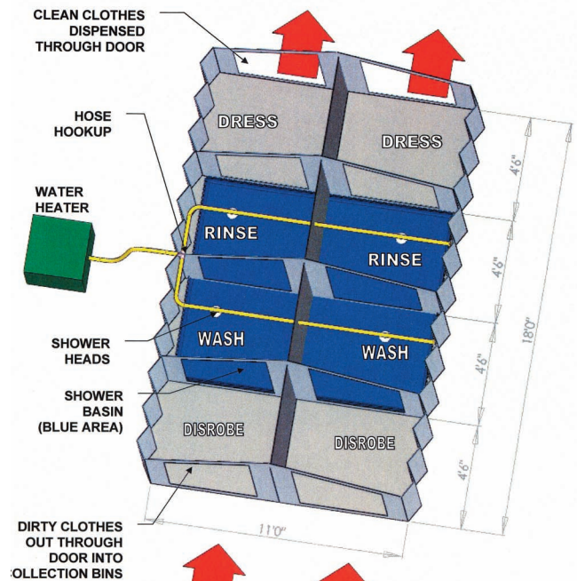
Decon Shower Assembly comes in 2 or 3 lane units.
